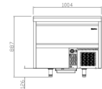
EB1000II
