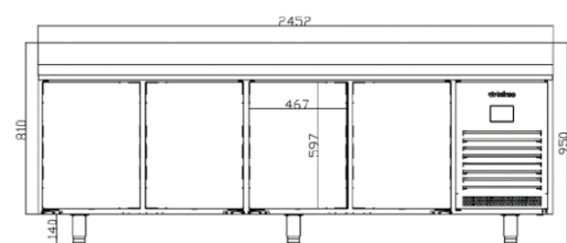
BMPPF2000II
