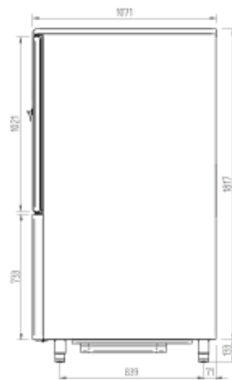
PERFIL/RIGHT VIEW/VUE EN PLAN
