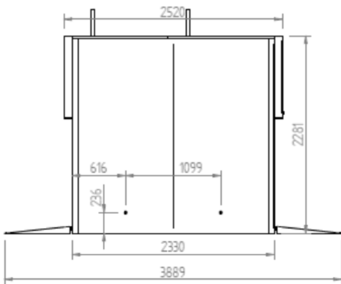
PERFIL/RIGHT VIEW/VUE EN PLAN
