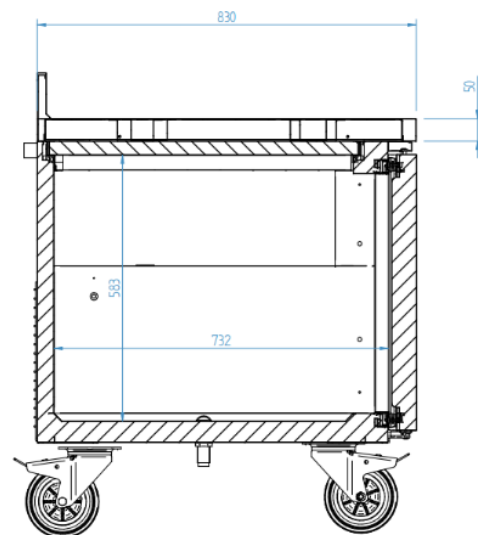
PERFIL/RIGHT VIEW/VUE EN PLAN
